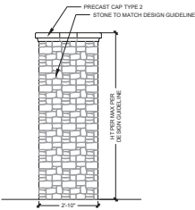
ELEVATION 2 COLUMN 3/8" = 1'-0"
