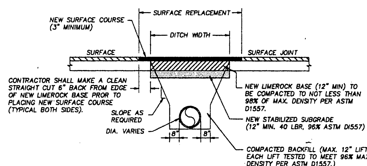
TRENCH WIDTH PAVEMENT REPLACEMENT
