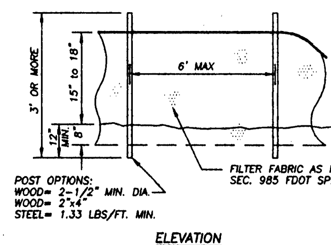
TYPE III SILT FENCE DETAIL FOOT INDEX #102
