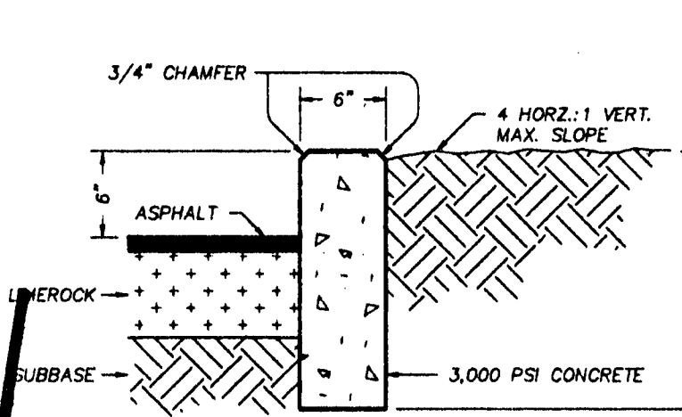
BARRIER CURB DETAIL SCALE: 1" = 1'
