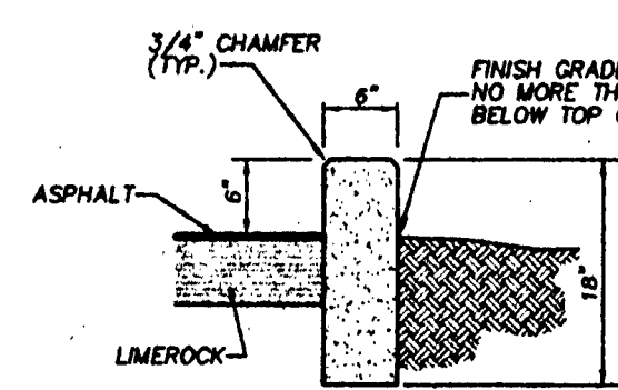
BARRIER CURB DETAIL
