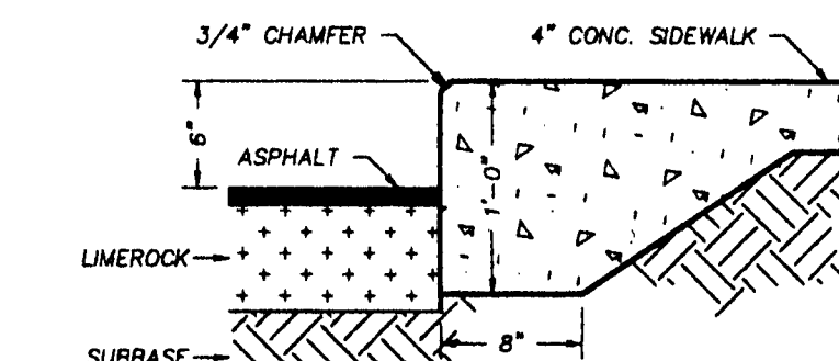
SIDEWALK & PAVEMENT DETAIL SCALE: 1" = 1'
