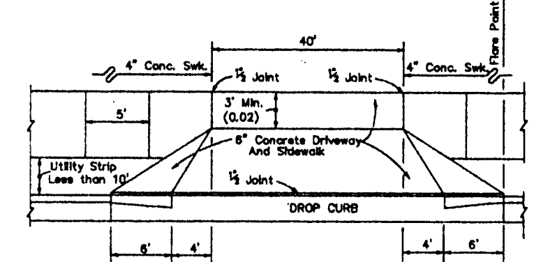
DRIVEWAY DETAIL
