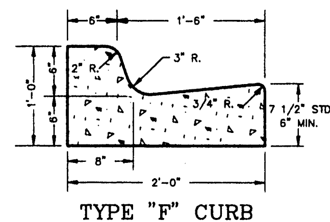
TYPE "F" CURB
