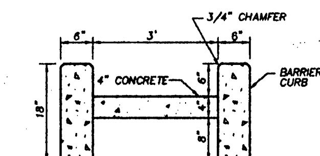
CONCRETE CHANNEL DETAIL
