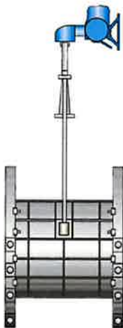
MXb and bevel gearbox mounted to sluice gate
