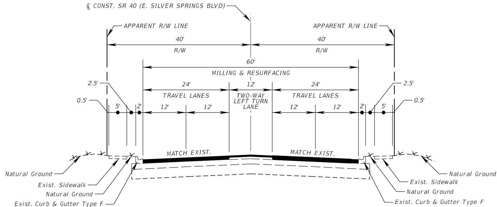
TYPICAL SECTION SR 40 STA. 1019+06.49 TO STA. 1124+39.67
