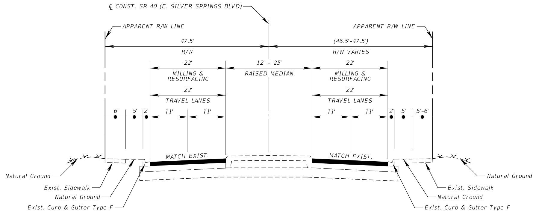
TYPICAL SECTION SR 40 STA. 1000+96.95 TO STA. 1019+06.49
