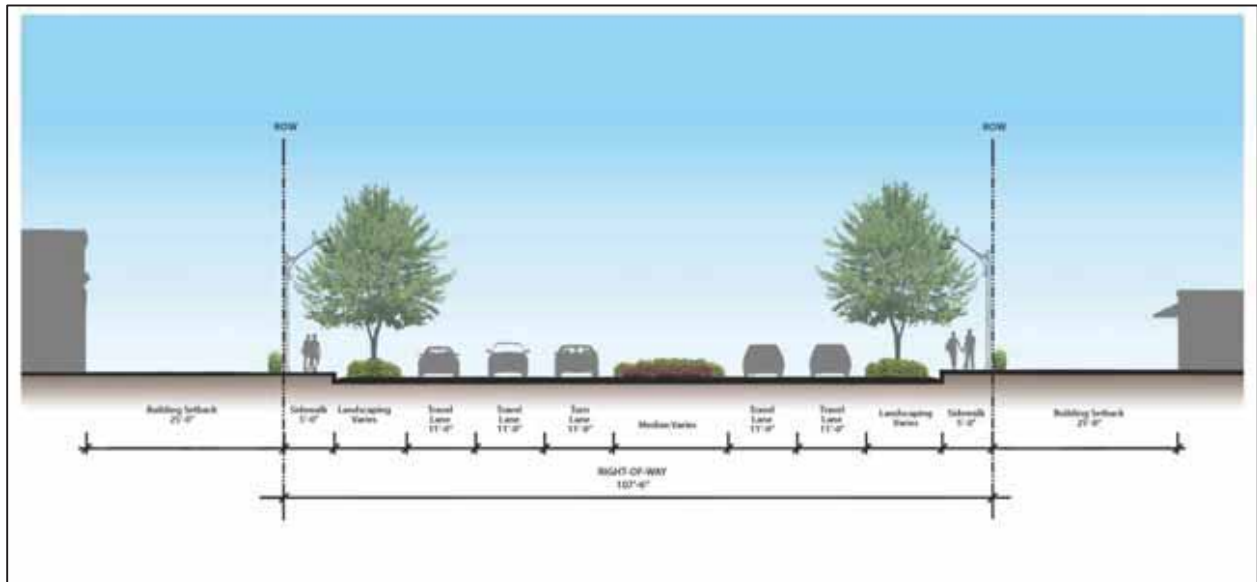
Cross-section with building setback of 25 feet
