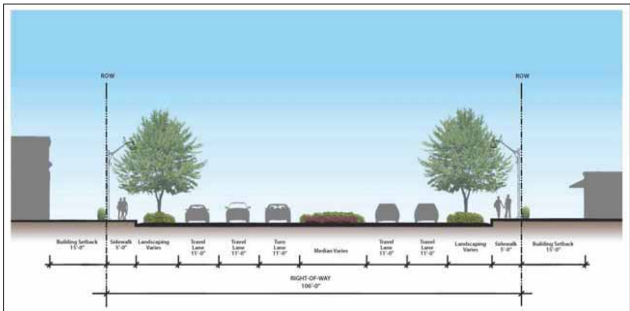
Cross-section with building setback of 15 feet
