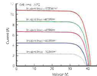
Current-Voltage Curve (LR4-60HPH-360M)
