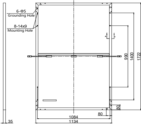
Mounting Hole
