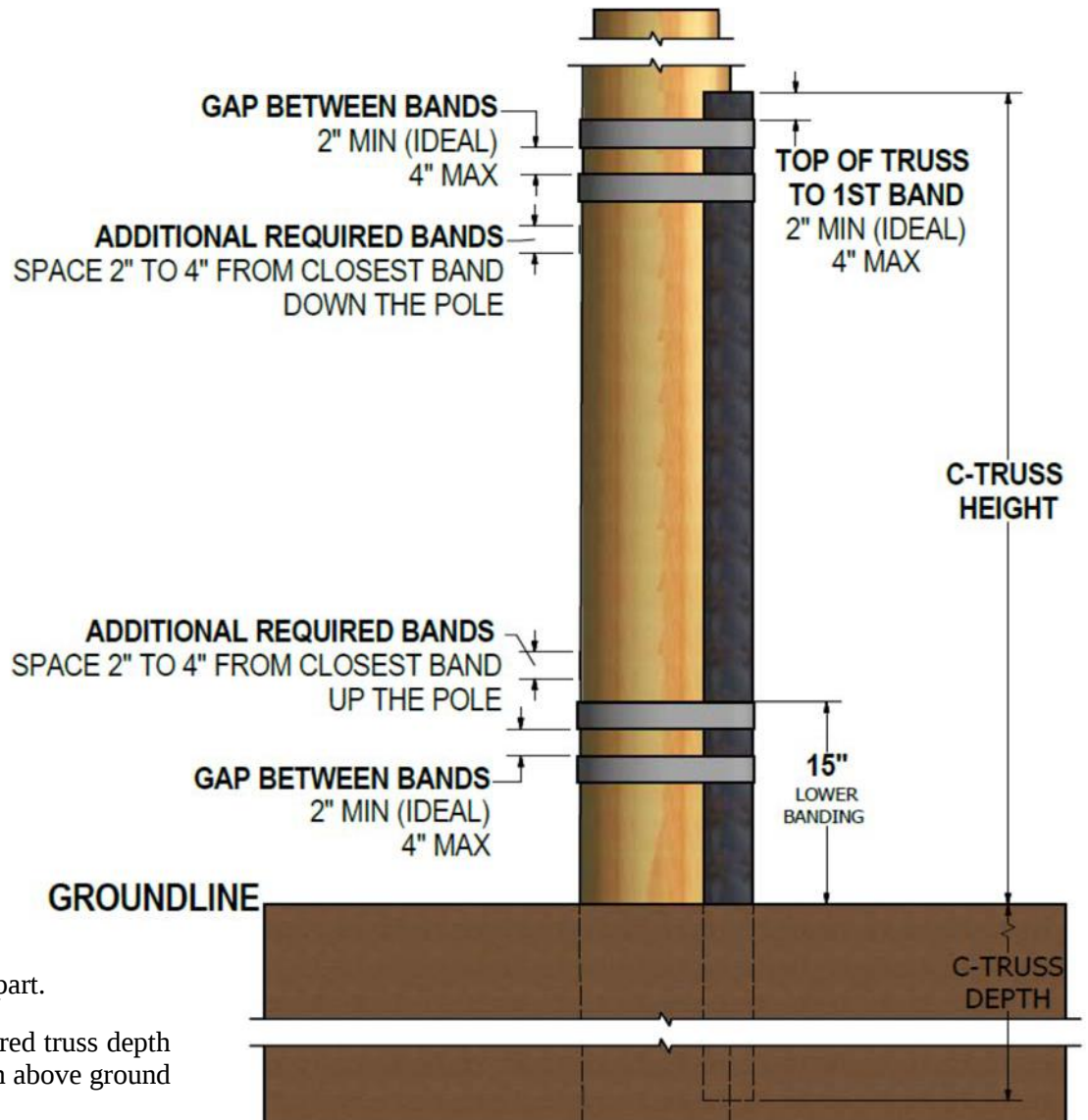
C-Truss and C2-Truss™ and Banding – Single Truss Installation Diagram
