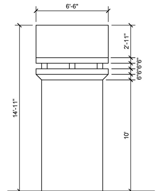
SIDE ELEVATION
