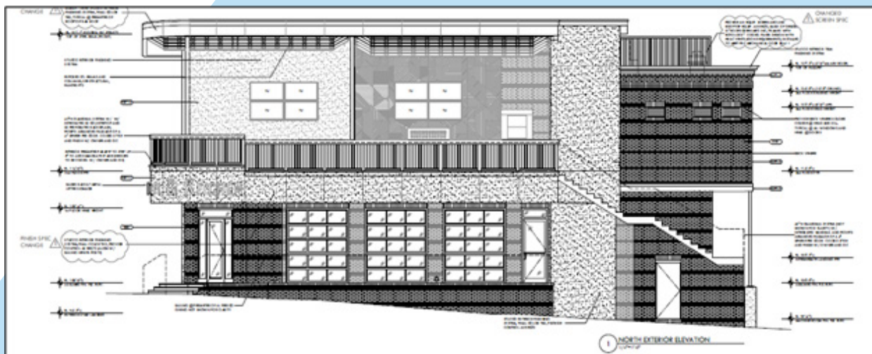
North Elevation
