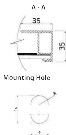
Frame Cross Section
