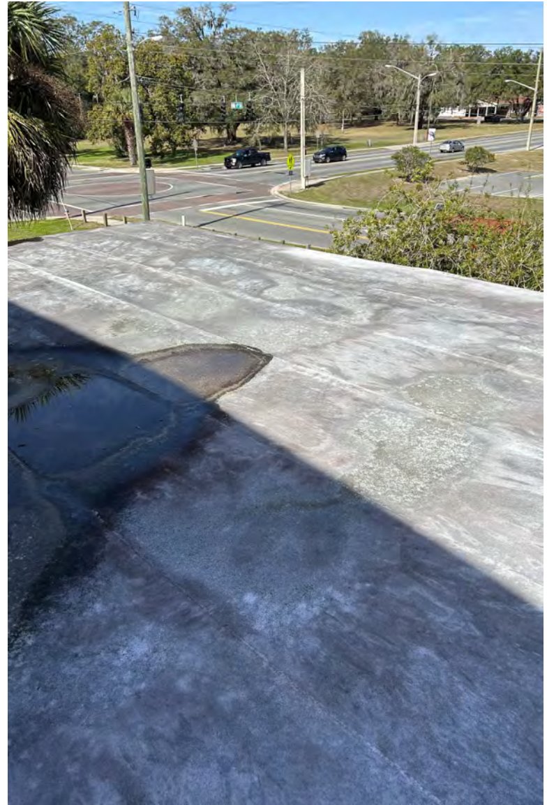
Ponding Water
