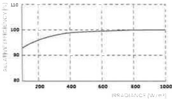
Typical module performance under low irradiance conditions in comparison to STC conditions (25 °C, 1000 W/m²)
