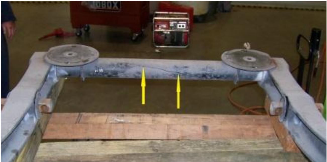
CRACKED TRANSVERSE BAR IN REAR, LOWER CONTROL ARM ASSEMBLY (3,785 TEST MILES)
