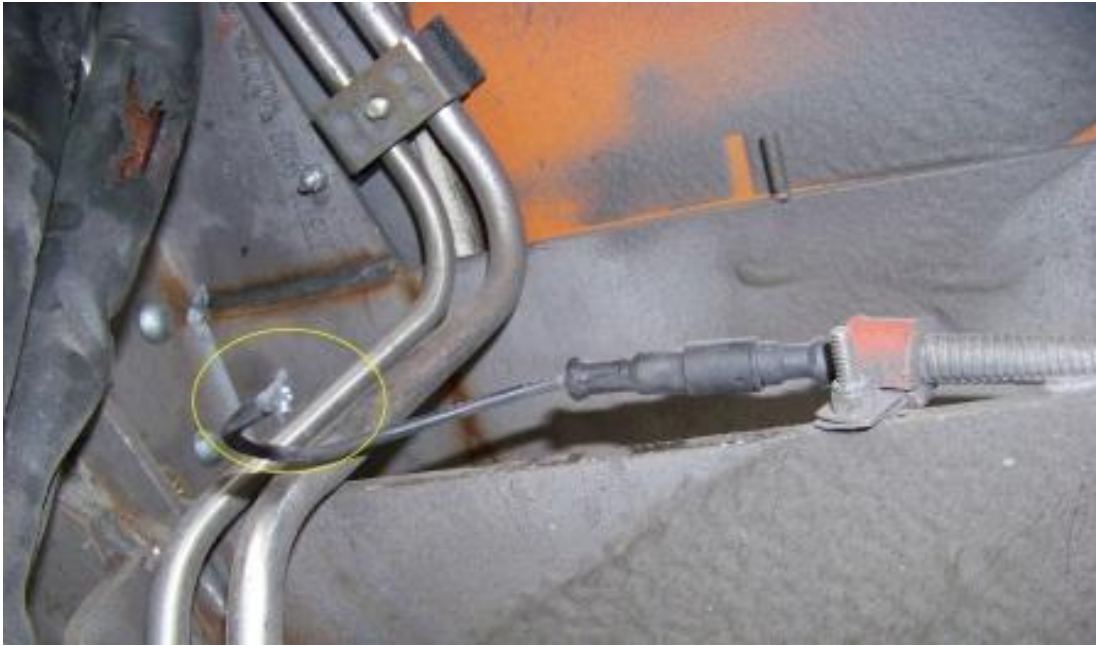
BROKEN LEFT REAR ABS SENSOR (5,451 TEST MILES)
