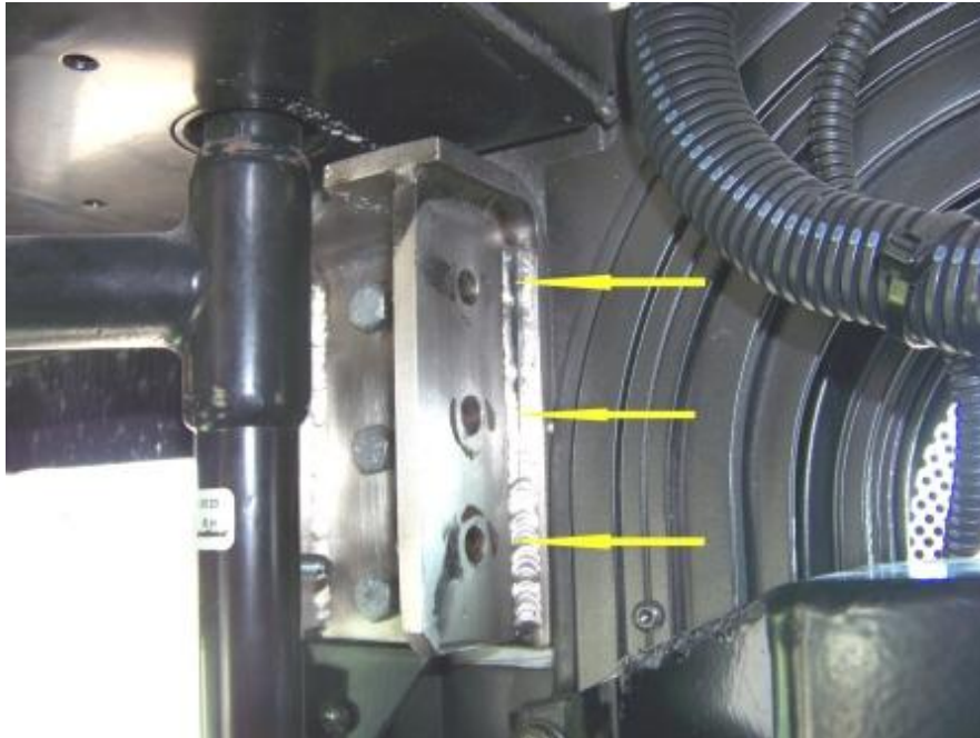
BROKEN BOLTS FRONT DOOR; UPPER SUPPORT BRACKET (13,877 TEST MILES)
